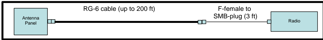
Figure 2: Electrical Connections
